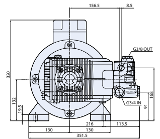
GR. 132 S motor hollow shaft
