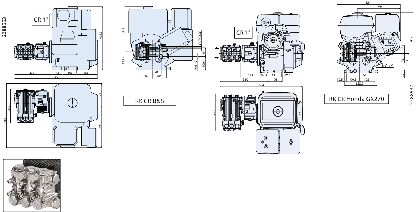
RK 15.15 CR S (Honda engine)
