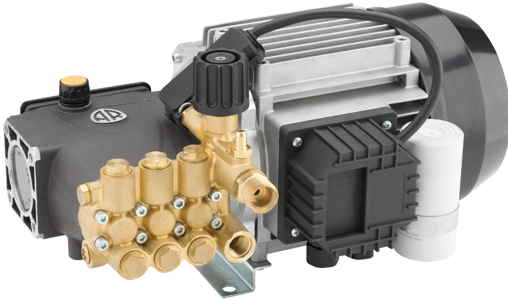
GR. 80 AR motor hollow shaft
