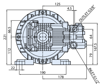
GR. 112 motor hollow shaft
