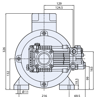
GR. 132 S motor hollow shaft
