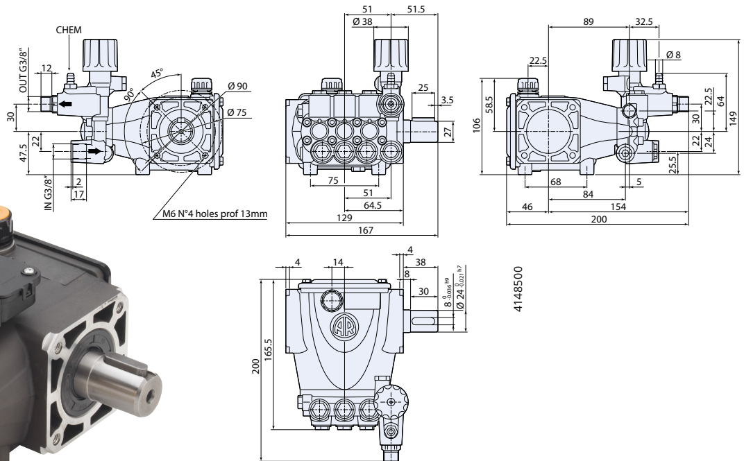
TSS version
